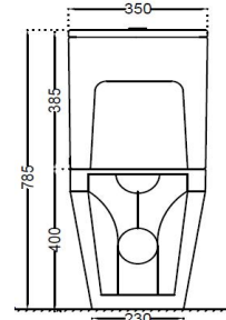
BACK VIEW
