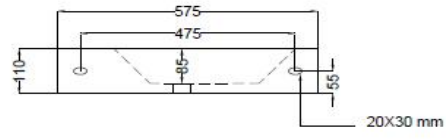
BACK VIEW
