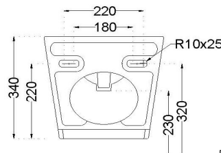
BACK VIEW
