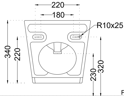
BACK VIEW
