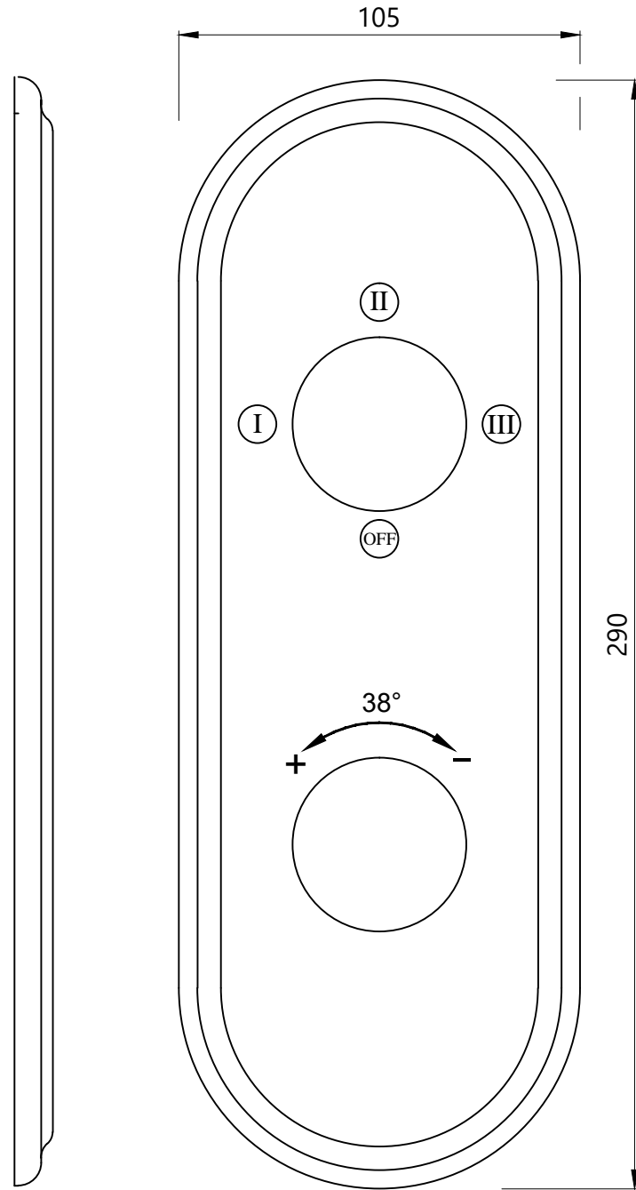
WALL FLANGE
