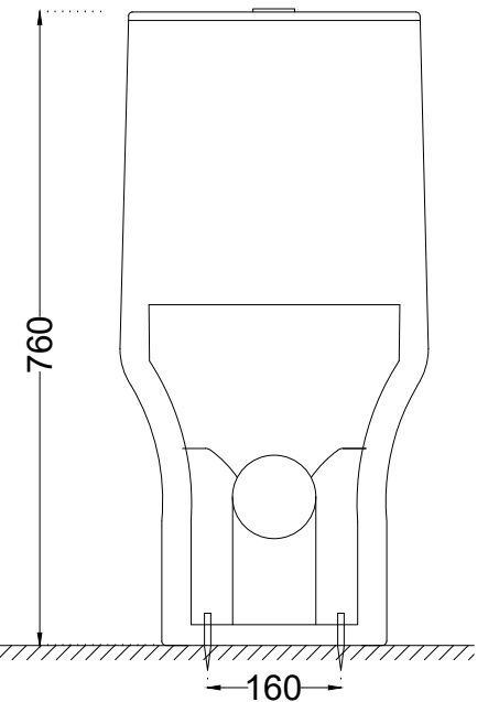
BACK VIEW
