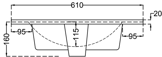
BACK VIEW
