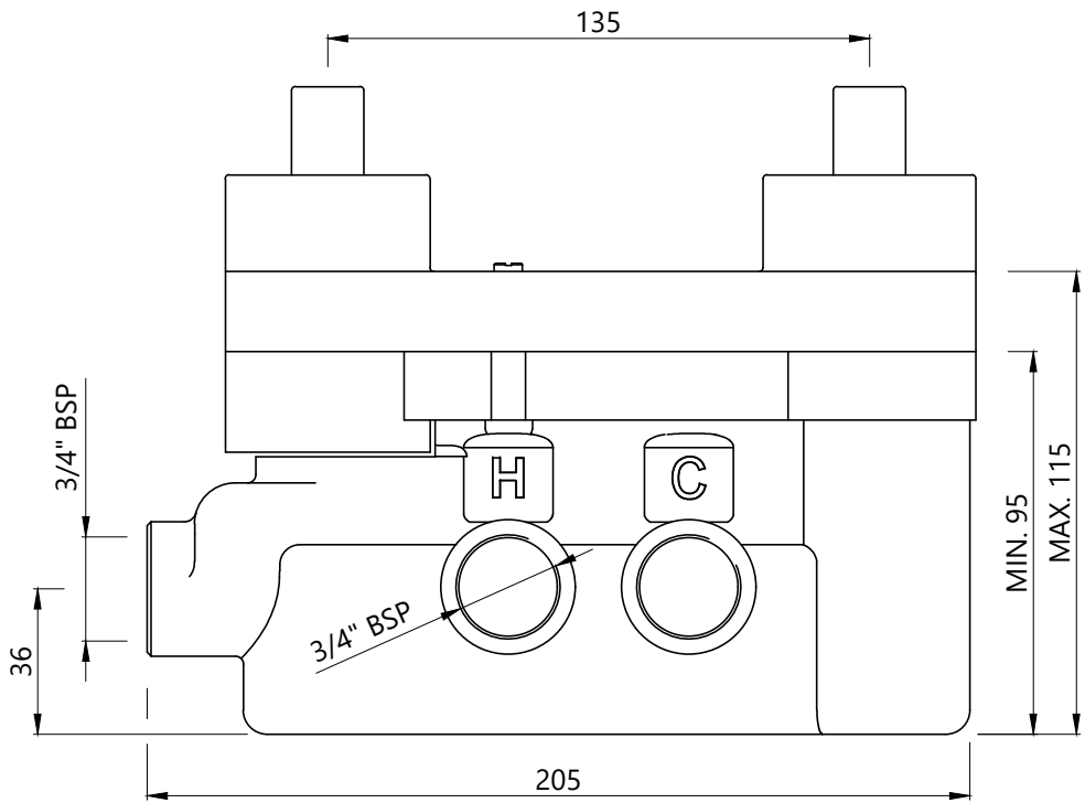
THERMOSTATIC SHOWER MIXER BODY
