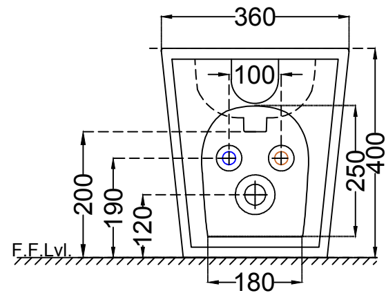
BACK VIEW
