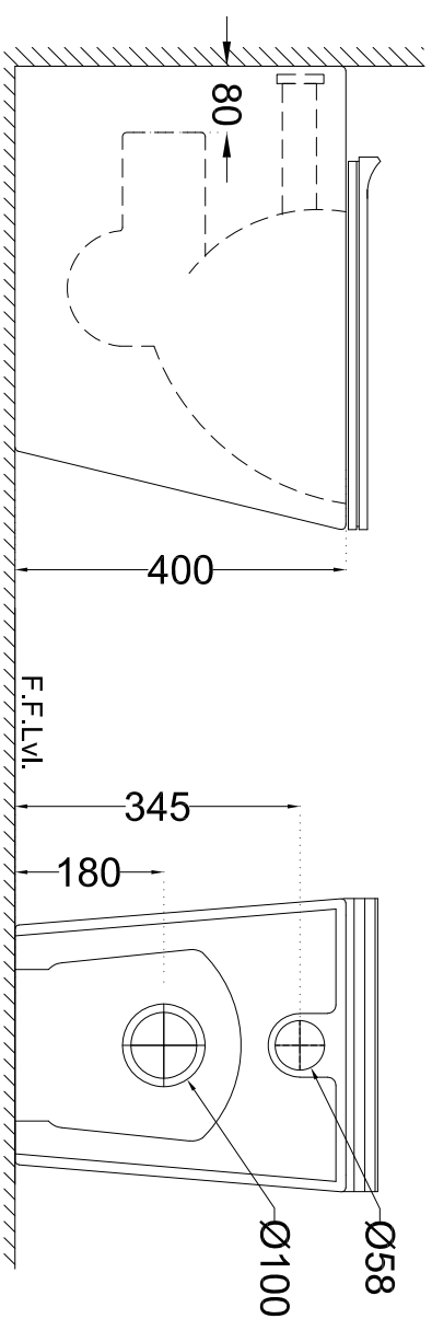
SIDE VIEW
