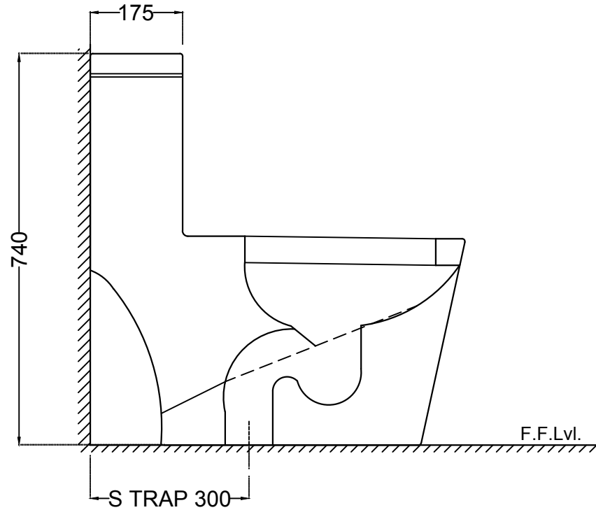
SIDE VIEW
