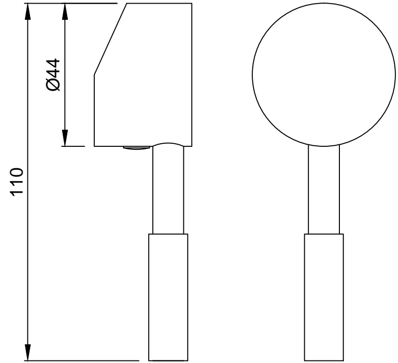
OPERATING LEVER
