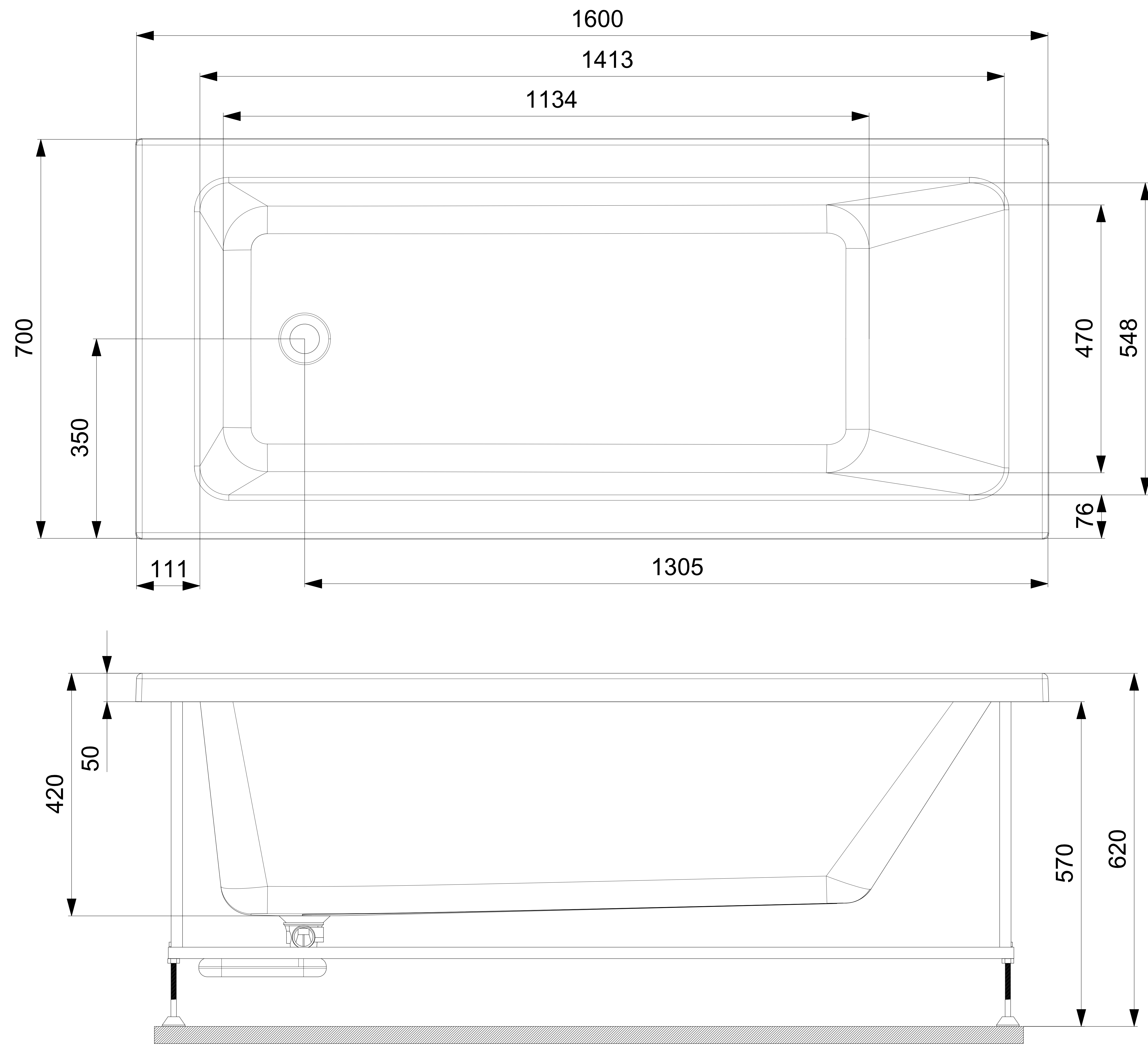
JBT-WHT-FONT160FX = FONTE 1600X700X420 BUILT IN BATHTUB WITH POWDER COATED MS FRAME
